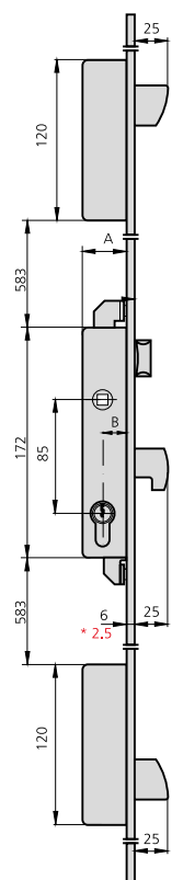
U-SHAPED FRONT PLATE
